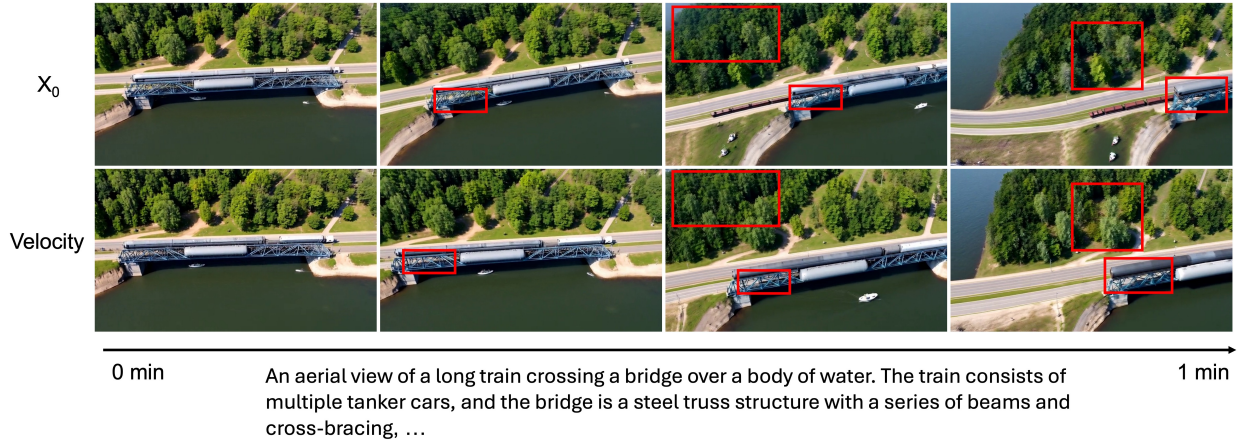
Figure 5: Velocity versus clean-latent matching. We compare distillation in the predicted clean-latent ( x_0 ) space and in the native velocity space over a one-minute rollout. Both variants remain plausible at the beginning, but x_0 matching progressively smooths fine structures and introduces geometric degradation in the bridge truss and foliage. Velocity matching better preserves these details at later timestamps. Red boxes highlight representative regions.
